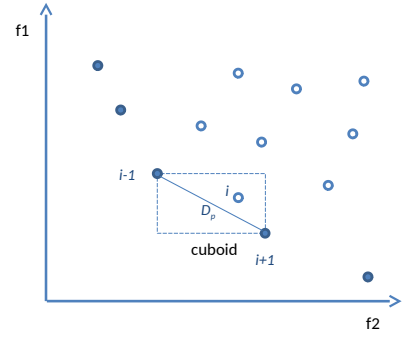
FIGURE 4. Crowding-distance calculation.
