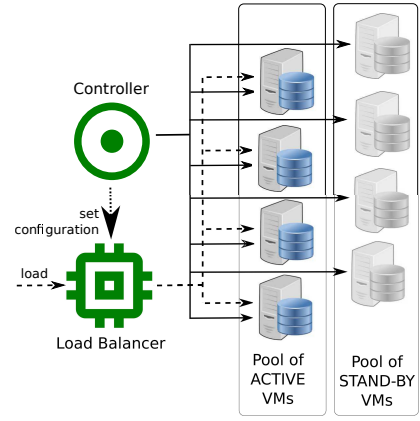
Figure 2. Internal architecture of a Cloud Region
