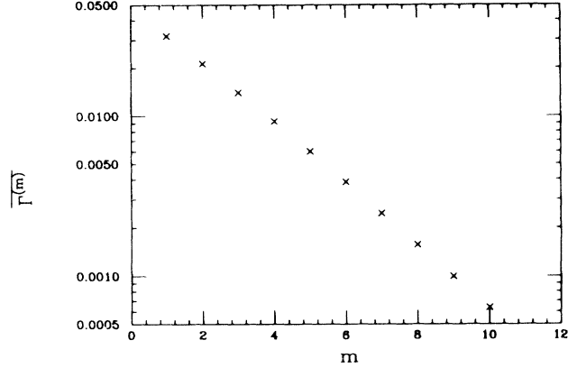
FIG. 2. \Gamma^{(m)} vs m using a log-linear scale for the random field Ising model with the same parameters of Fig. 1.
