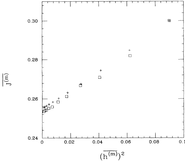
FIG. 1. Random field Ising model with constant J=0.3 and h=0.2 or h=0.4 with equal probability. Flow of [h^{(m)}]^2 , J^{(m)} for m=0,1,\dots,10 (squares). The fixed point is h^*=0 , J^*=0.253 . For comparison, there is also the corresponding flow for the Ising model with constant field and coupling J=0.3 , h=0.3 (crosses).
