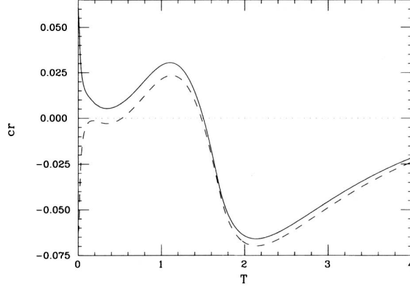
Fig. 5. Horizontal first neighbors correlation cr = \overline{\langle \sigma_{i,j} \sigma_{i,j+1} \rangle} for the P(l) = a_l/(l+q)^3 case. The parameter is q = 1 , the horizontal coupling is J_h = 0.3 , the vertical couplings are J_v = 1.49 (full) and J_v = 1.51 (dash).
