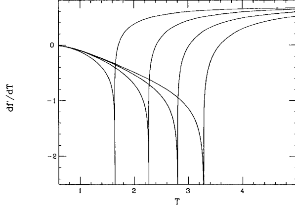
Fig. 2. Temperature derivative df'/dT of f' \equiv [\partial f / \partial p]_{p=0} as function of T . The horizontal coupling is J_h = 1 , the different lines correspond to the vertical couplings J_v = 0.5 , J_v = 1 , J_v = 1.5 and J_v = 2 .
