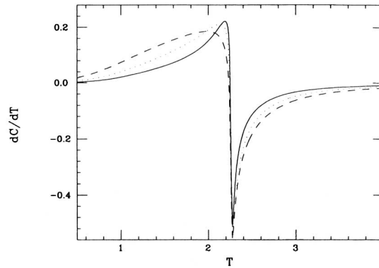
Fig. 4. Temperature derivative (1/\bar{l})(dC/dT) of the specific heat function of the temperature T for the P(l) = a/(l+q)^3 case. The couplings are J_h = 1 and J_r = 1 . The values of the parameter are q = 10 (full), q = 5 (dots), q = 2 (dash).
