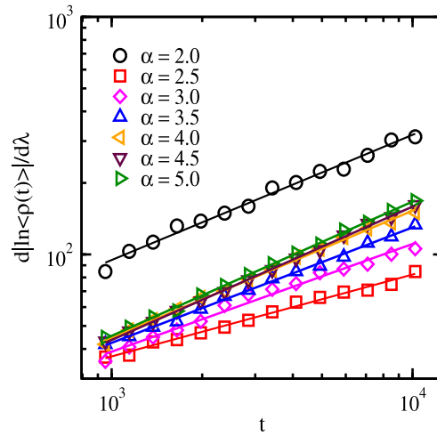
Fig. 5. Log–log plot of the derivative of d|\ln\langle\rho(t)\rangle|/d\lambda versus time t at the critical point for a system of size L = 10000 . The best fit gives the critical exponent ratio 1/z\nu_{\perp} .
