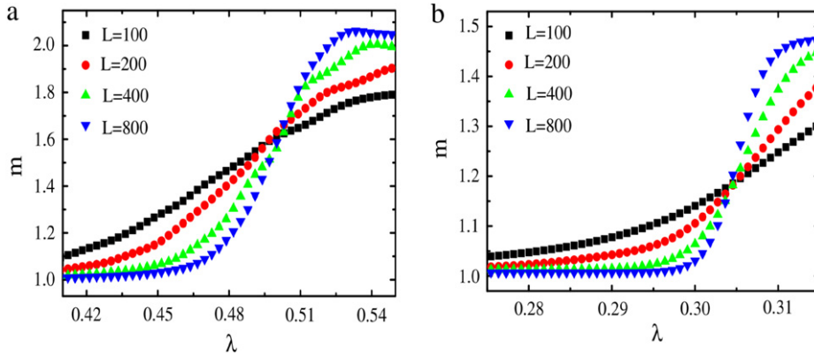
Fig. 2. (Color online) The moment ratio m as a function of the control parameter \lambda for different sizes L . All curves intersect in the critical point, giving an estimation for \lambda_c ; (a) \alpha = 2.0 \rightarrow \lambda_c = 0.5071 ; (b) \alpha = 5.0 \rightarrow \lambda_c = 0.3065 .
