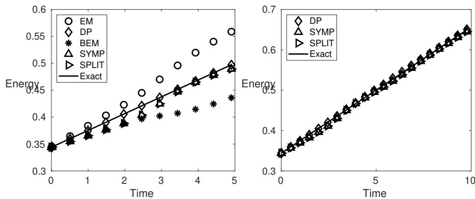
FIGURE 4. Numerical trace formulas for the stochastic mathematical pendulum on [0, 5] (left) and [0, 10] (right).
