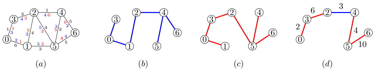
Figure 1: (a) An example of all the potential tunnels that could have been built by the two companies. Tunnel lengths are in black while tunnel costs for the first and second company are in blue and red, respectively. (b) The subway network built by the first company. (c) The subway network built by the second company. (d) The quickest route from location 0 to location n - 1 when t_1 = 3 and t_2 = 2 . Black numbers refer to travel times.
